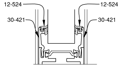
1" GLAZING
