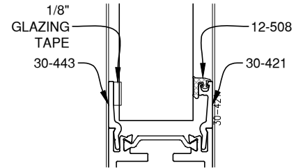
1 3/16" GLAZING
