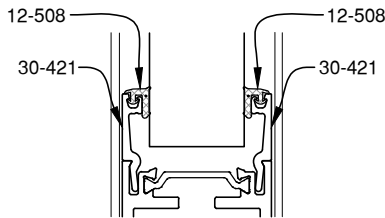
1 1/16" GLAZING
