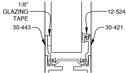
1 1/8" GLAZING
