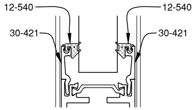
7/8" GLAZING
