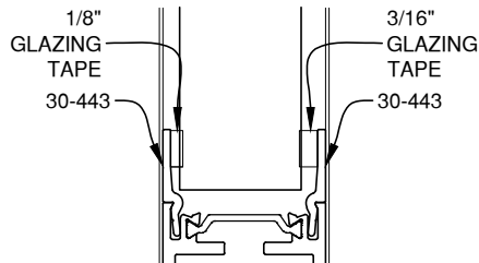
1 1/4" GLAZING
