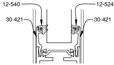
15/16" GLAZING
