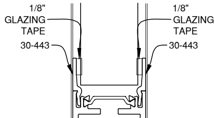
1 5/16" GLAZING
