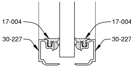
1/2" GLAZING
