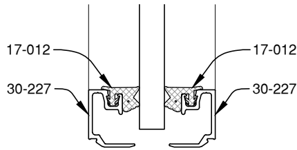
3/8" GLAZING
