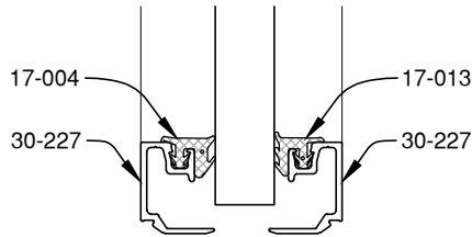
9/16" GLAZING
