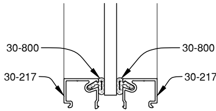
1/4" GLAZING
