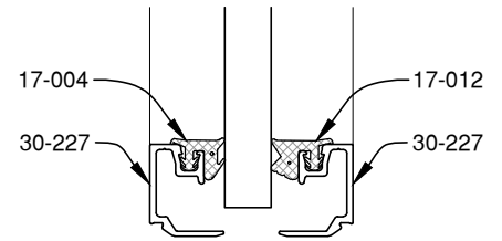
7/16" GLAZING
