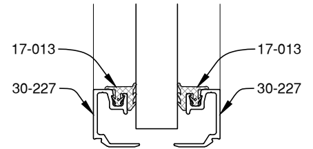
5/8" GLAZING
